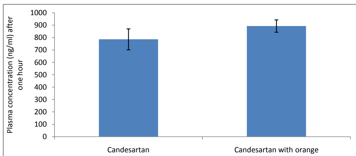
Figure 16: Diagram with error bars comparing the mean (with its 95% confidence interval) serum candesartan drug concentration after one hour of drug administration between single and combined drug use.
